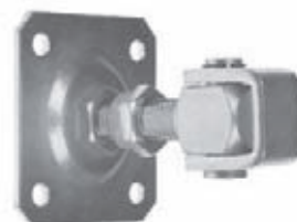
adjustable hinges with shield M16, 80 x 80 x 3
